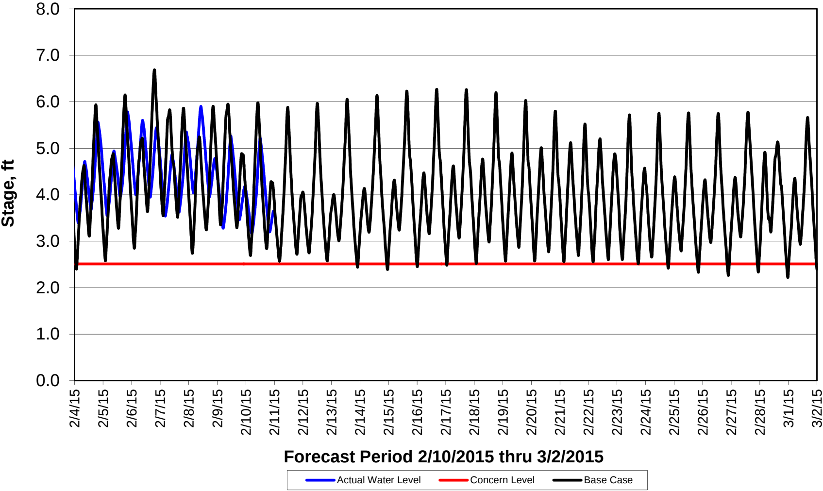
Forecasted Stage Middle River @ Howard Road
