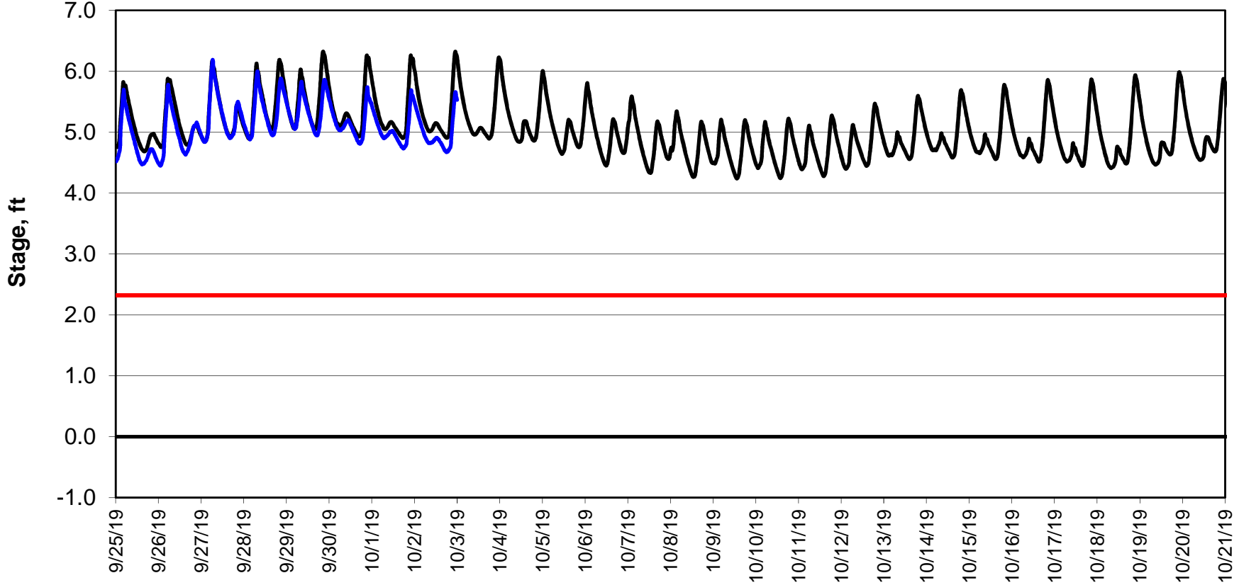
Simulation Period 9/25/2019 thru 10/21/2019
