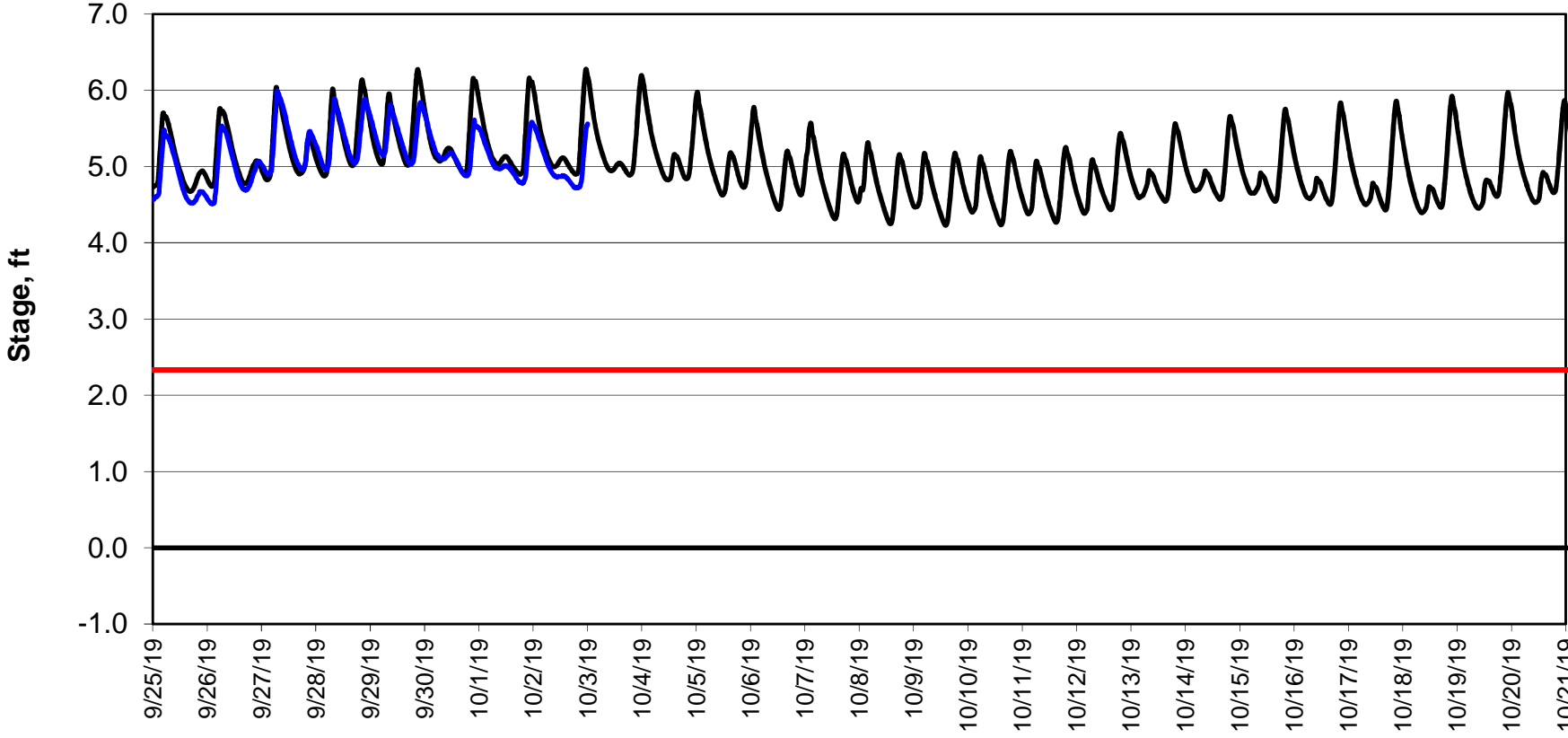
Simulation Period 9/25/2019 thru 10/21/2019 — Base Case — Observed Water Level — Concern Level
