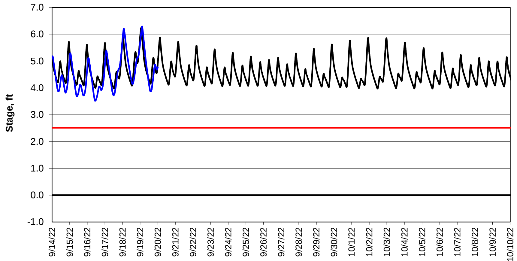
Forecasted Stage Middle River @ Howard Road
