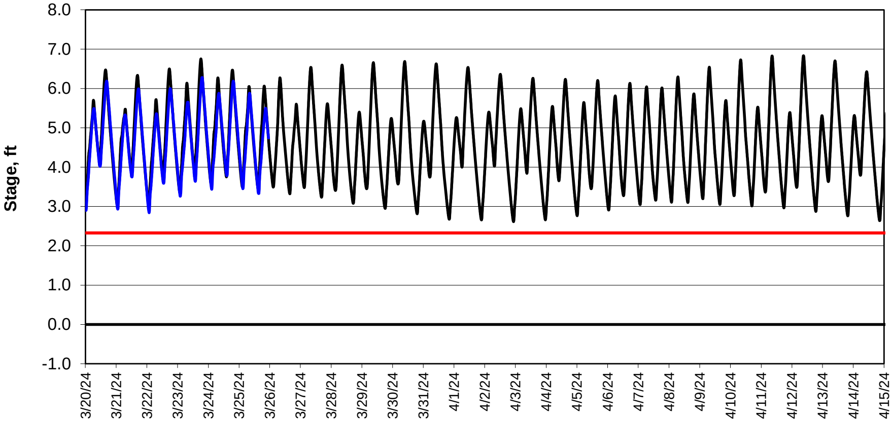
Simulation Period 3/20/2024 thru 4/15/2024
