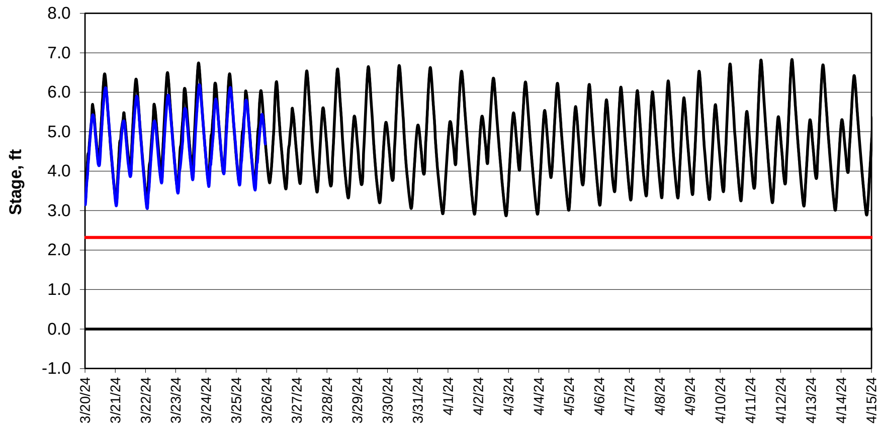
Forecasted Stage @ Doughty Ct/Channel 205
