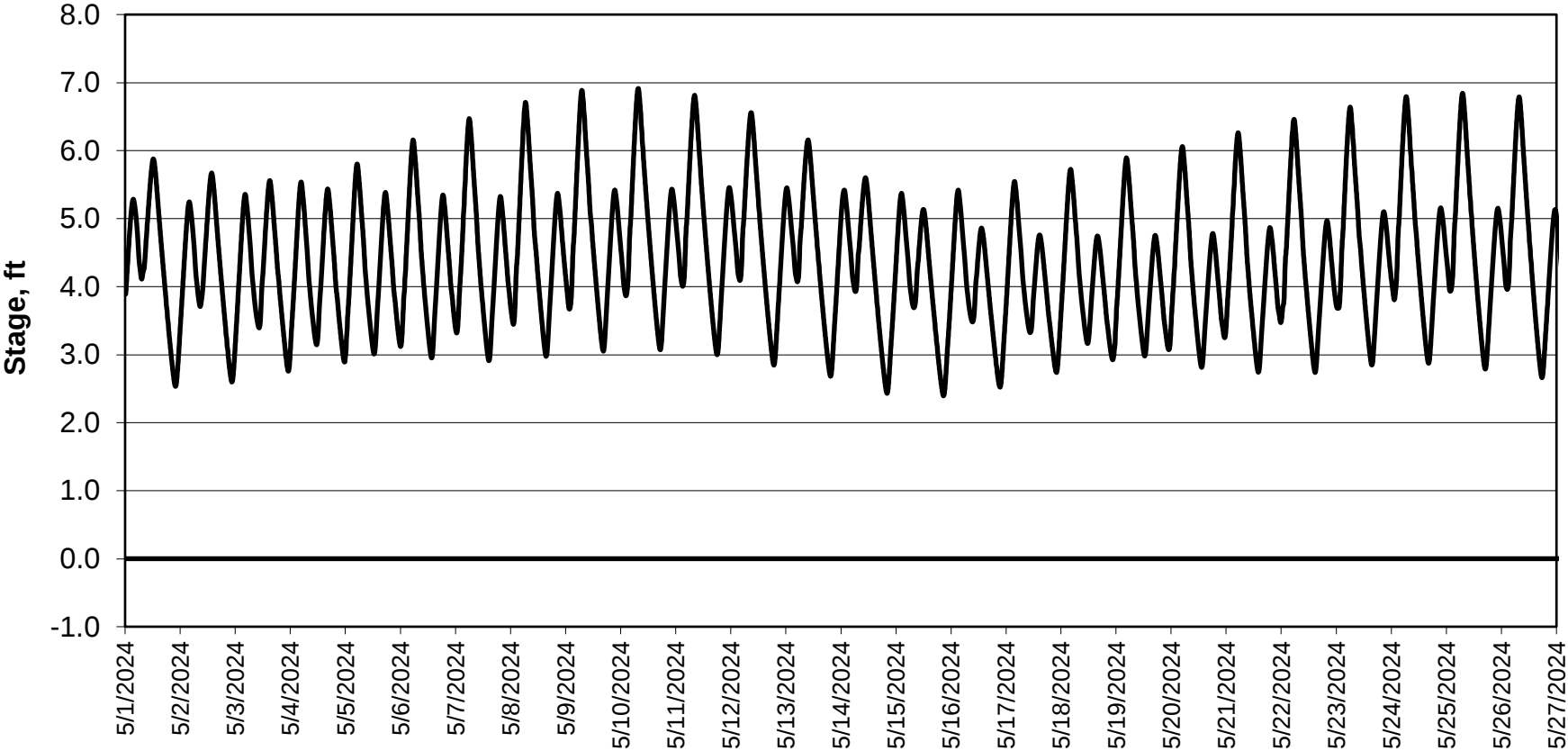
Forecasted Stage @ East End of Grant Line Canal/Channel 204
