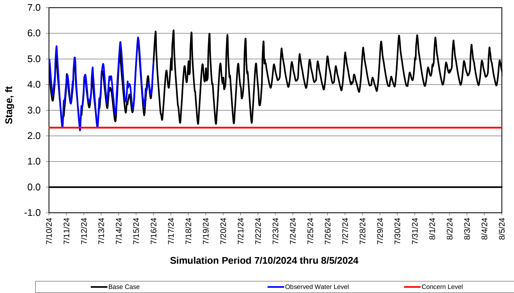
Forecasted Stage @ Doughty Ct/Channel 205
