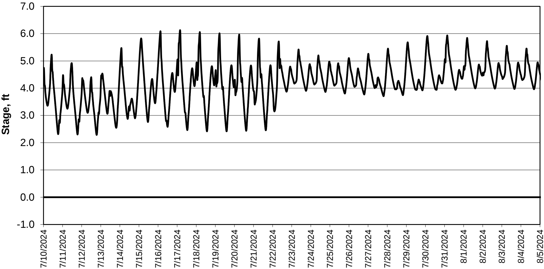
Forecasted Stage @ East End of Grant Line Canal/Channel 204
