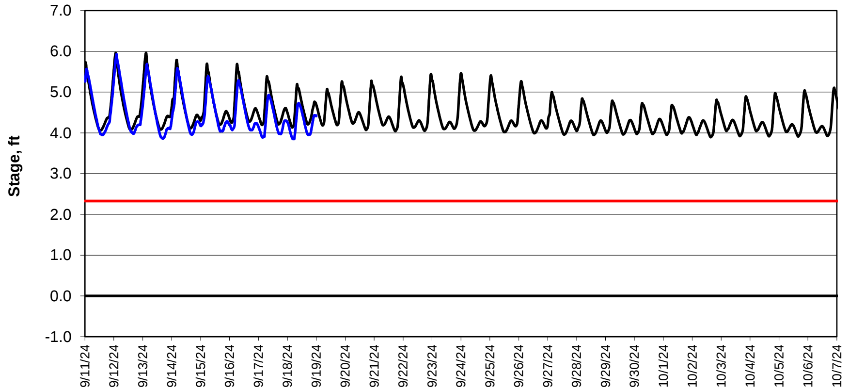
Forecasted Stage @ Old River @ Tracy Road
