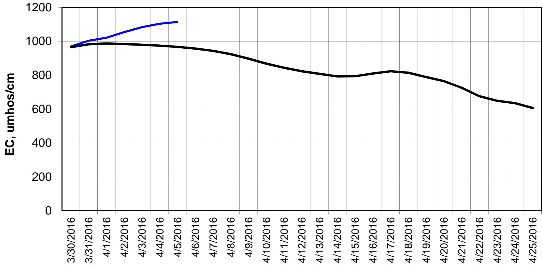
Simulation Period 3/30/2016 thru 4/25/2016 — Hist EC — Base Case
