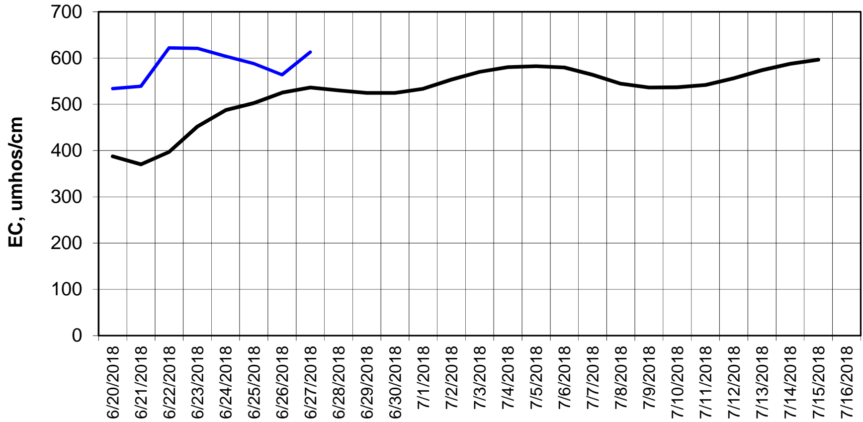
Simulation Period 6/20/2018 thru 7/16/2018 — Observed EC — Base Case
