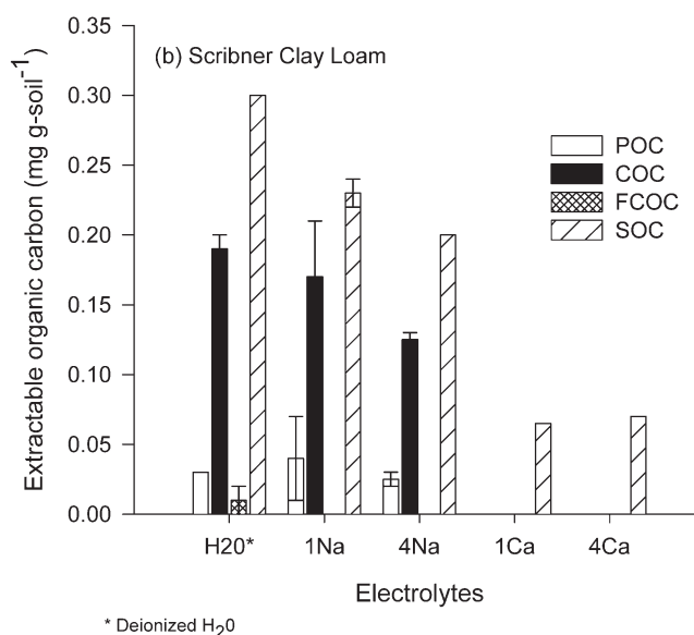
Fig. 4. Quantities of extractable organic C by different electrolytes. H 2 O, deionized H 2 O; POC, particulate organic carbon; COC, colloidal organic carbon; FCOC, fine colloidal organic carbon; SOC, soluble organic carbon. 1Na and 4Na represent Na-based electrolytes with electrical conductivity of 1 and 4 dS m -1 , respectively. 1Ca and 4Ca indicate Ca-based electrolytes with electrical conductivity of 1 and 4 dS m -1 , respectively.
