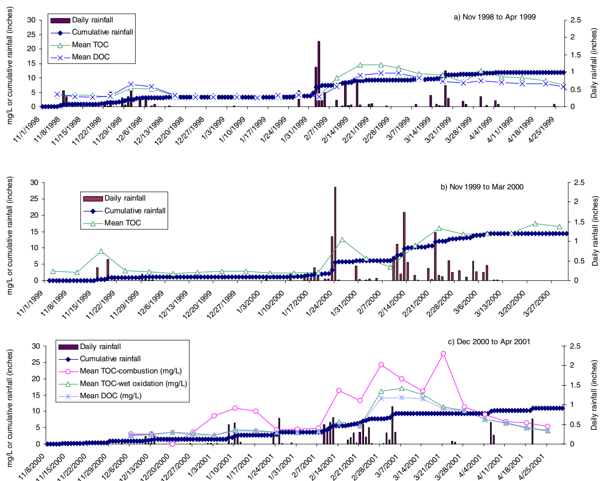
Figure 14 Comparison of TOC/DOC vs. rainfall at the Barker Slough Pumping Plant
