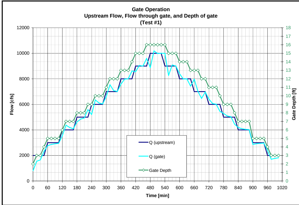
FIGURE1 Test 1: Upstream flow, flow through the gate, and depth of gate versus time.
