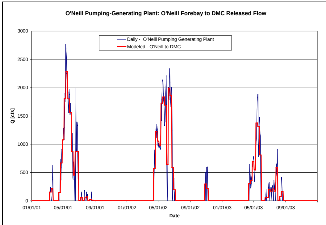
FIGURE 5-10 O'Neill Generating Plant Flow Data, Daily and 7-Day Average (DSM2 input)
