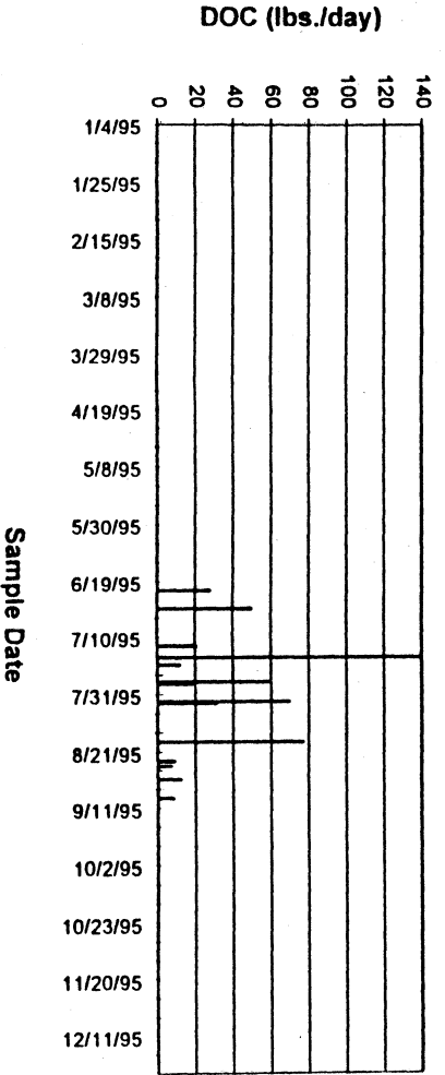
Figure 7. Mass Load of DOC from Siphons
