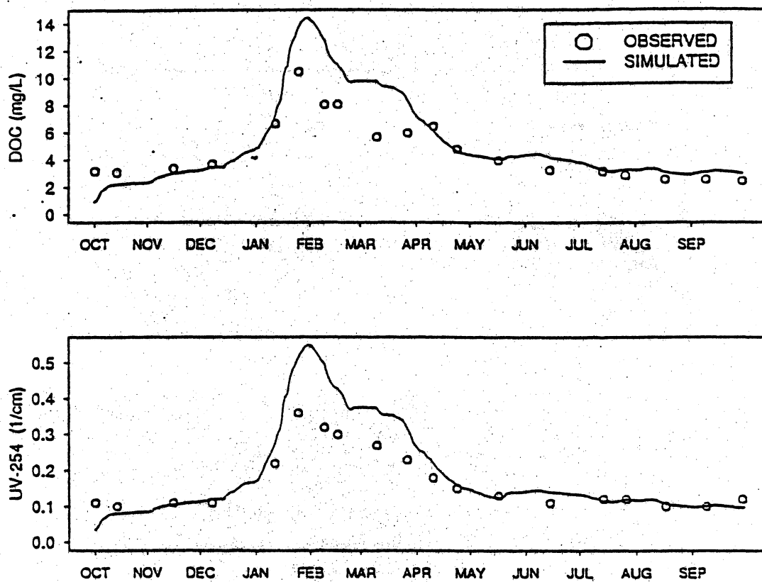
Simulated DBP Organic Precursor Time Series at Harvey O. Banks Pumping Plant: October 1, 1992 through September 30, 1993
