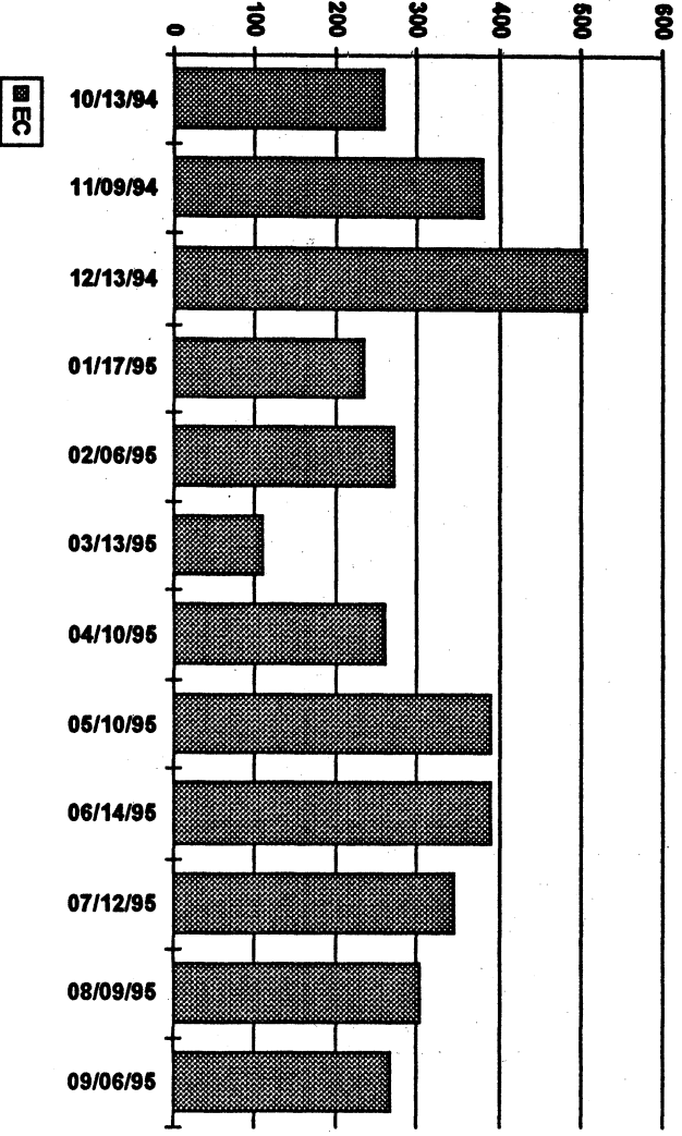
Figure 15. Barker North Bay EC
