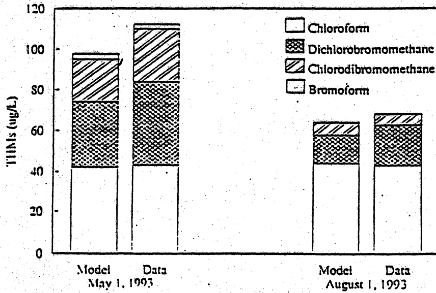
Simulated and Observed THM Concentrations at Harvey O. Banks Pumping Plant: May 1 and August 1, 1993
