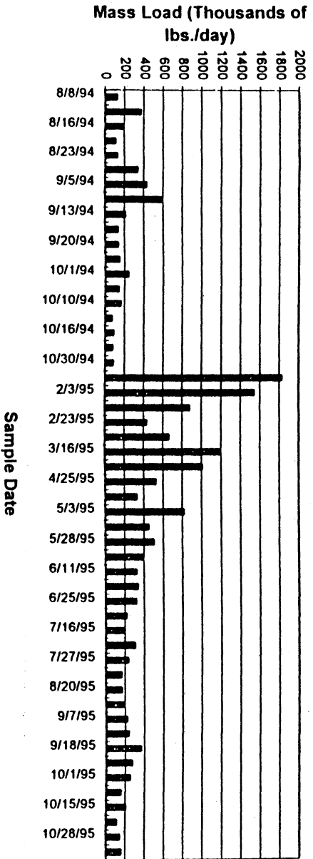
Figure 10. Mass Load of DOC in Sacramento River at Greeneres Landing
