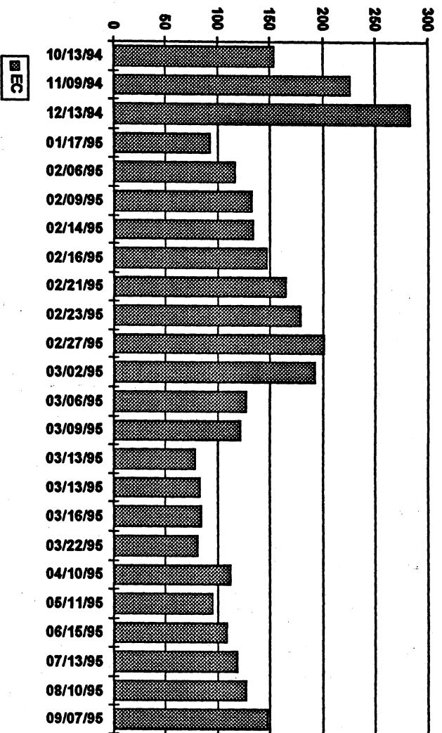
Figure 12. Sacramento River at Bryte Bend EC
