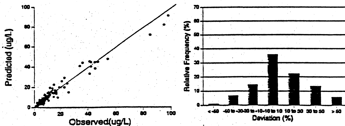
Chloroform Verification Results
