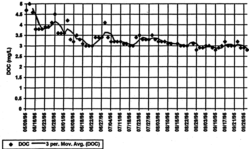
Figure 26. Harvey O. Banks Headworks DOC (mg/L)
