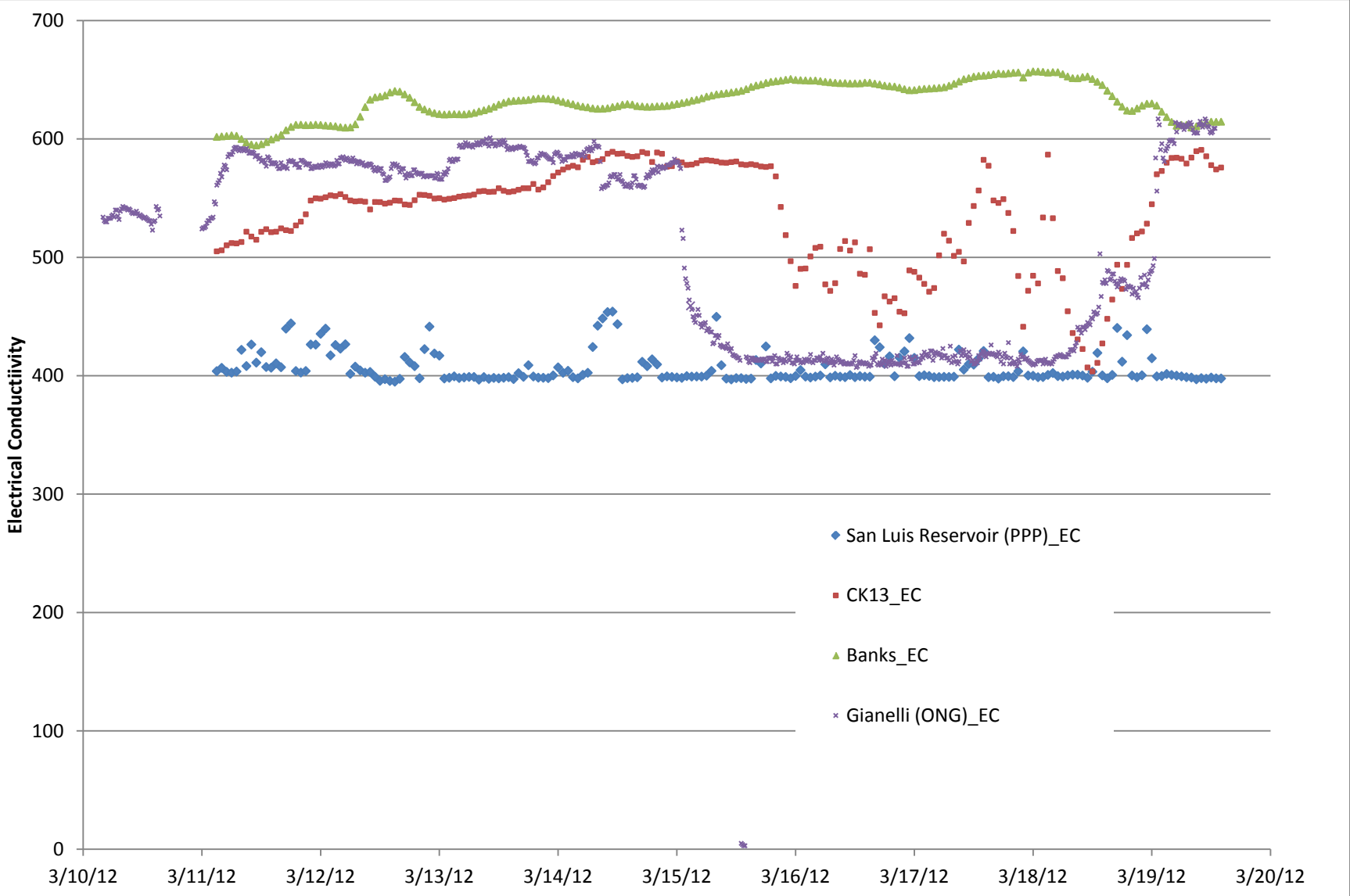
Electrical Conductivity signature at Gianelli Station with other EC data from source locations
